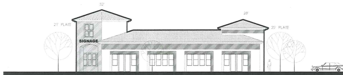
EAST ELEVATION
